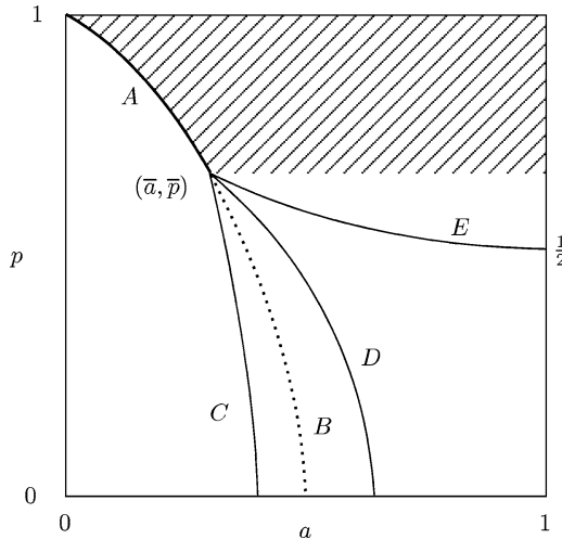
Fig. 1. The phase diagram of the q = 1 BCP model on the square lattice. The model may be transformed into the Ising model with edge-interaction J and external field h , see (4.3). The arc A \cup B with equation a/(1 - a) = 1 - p corresponds to h = 0 , and the points to its right (respectively, left) correspond to h > 0 (respectively, h < 0 ). There is a ‘tri-critical point’ at (\bar{a}, \bar{p}) , see (4.6), and the arc A joining this point to (0, 1) marks a line of first-order phase transitions. The region to the left of A \cup C is R(\Pi_{\text{icvc}}) , and that to the right of A \cup D is R(\Pi_{\text{iovc}}) . The hatched region lies in R(\Pi_{\text{icc}}) , and the lower boundary of R(\Pi_{\text{icc}}) is presumably as marked by E .
