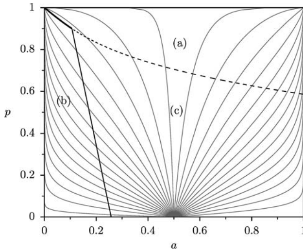
Fig. 2. The Blume–Capel phase diagram in two dimensions as proposed by Capel. Note the three phases labelled (a), (b), (c) as in the text. The boundary between (a) and (b) is thought to be a line of first-order phase transitions, whereas that between (a) and (c) is expected to be a line of second-order transitions. The point at which the phases are expected to meet is termed the tri-critical point . Moral support for such a phase diagram is provided by the rigorously known q = 1 diagram of Figure 1.
