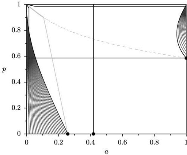
Fig. 3. Regions of the phase diagram of the Blume–Capel model on \mathbb{L}^2 about which one may make rigorous statements on the basis of comparisons with other models. The three points referred to in (i)–(iii) are marked. The narrow vertical strip along the p -axis is a subset of R(\Pi_{\text{icvc}}) , and the horizontal strip along the line p = 1 is a subset of R(\Pi_{\text{iec}}) ; see the comments around (9.1) and (9.2).
